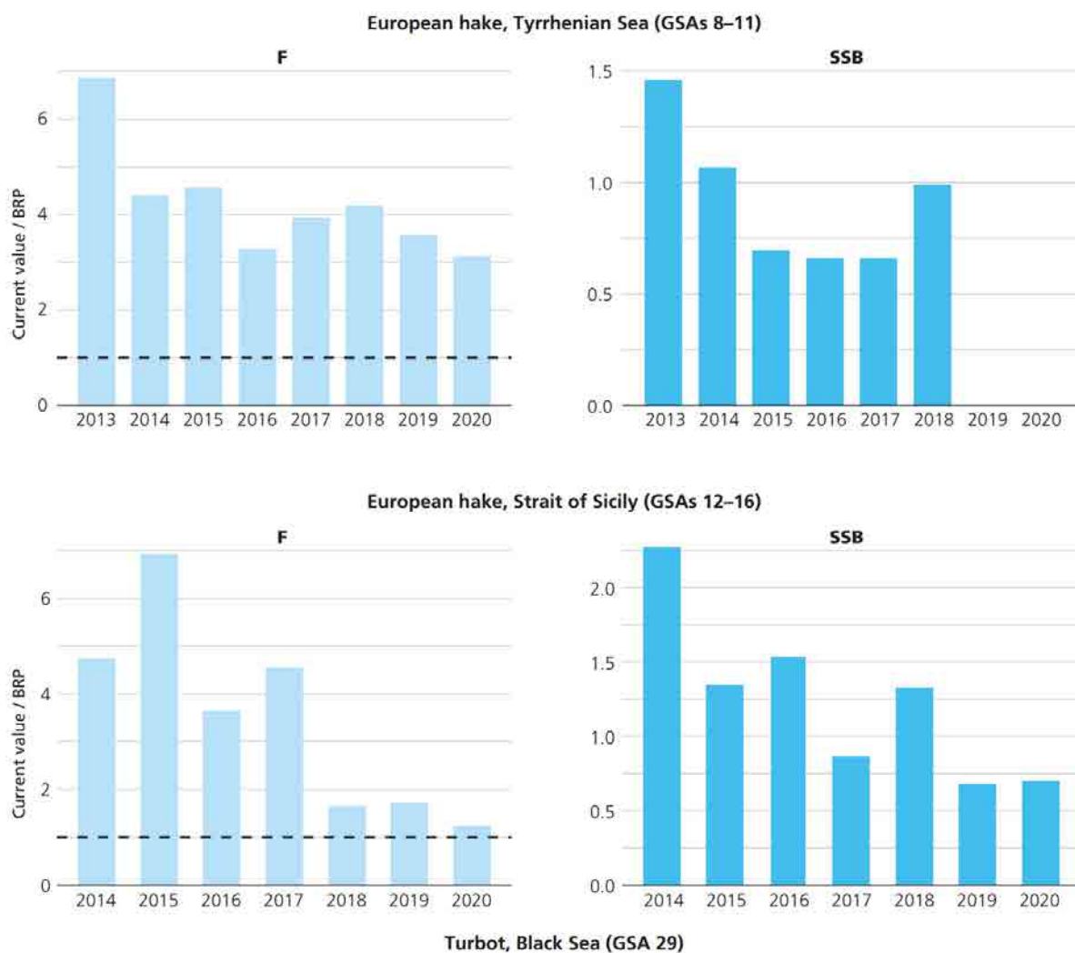
Figure 211: Annual progression in biomass (B/BPA) (right) and exploitation ratio (F/FMSY) (left) for European hake in the Tyrrhenian Sea and the Strait of Sicily
