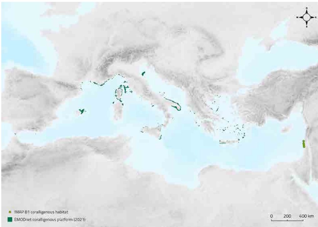
Figure 131: Distribution of Coralligenous habitat in the Mediterranean Sea (from EMODnet (2021) and location of monitoring sites for Coralligenous habitat, based on data reported under IMAP up to December 2022).
