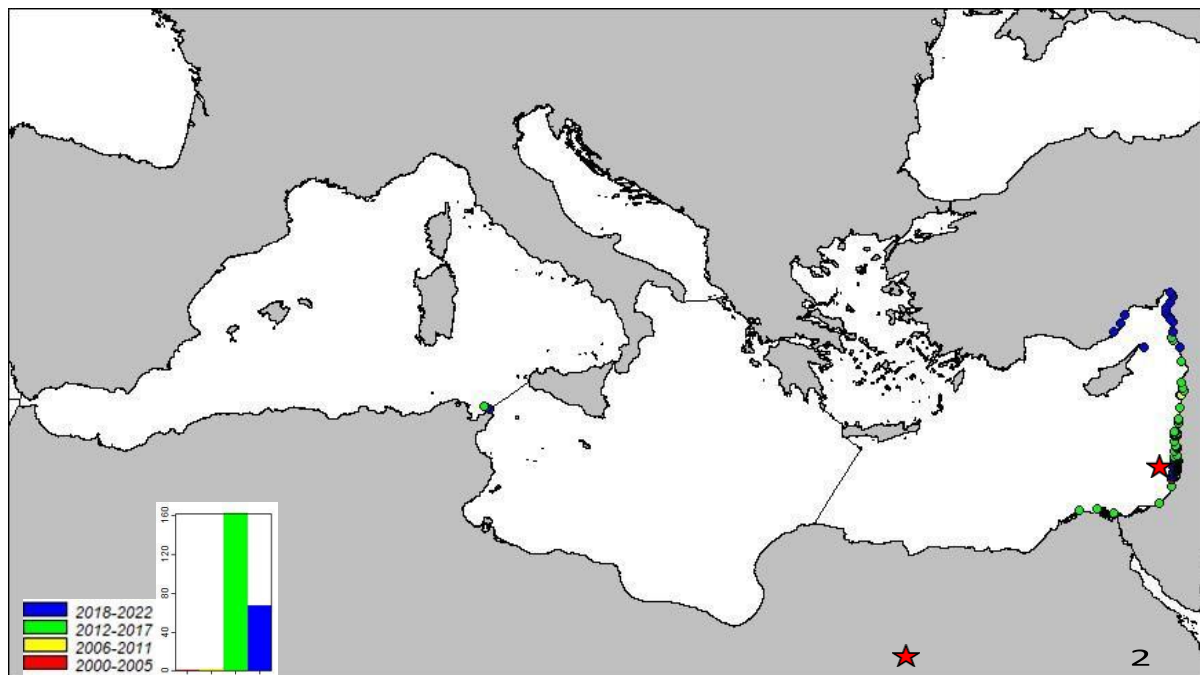
Figure 107: Distribution of Plotosus lineatus in the Mediterranean Sea. Details as in Figure105.
